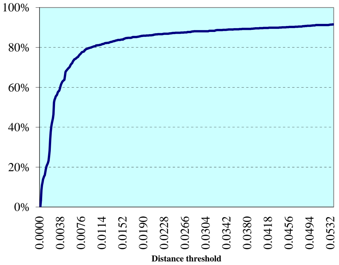
Figure 3 Percentage of cases matched with D(i, j) < \text{threshold}
